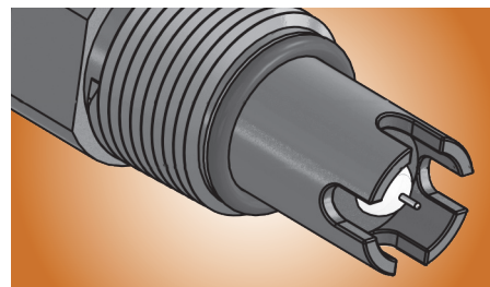
O94BPE Sensor Tip Detail
