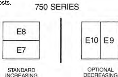
FIG. 3-2 750 SERIES DECREASING JUMPER CONVERSION
