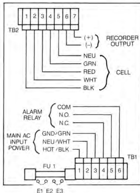
FIG. 2-4 750 SERIES INSTALLATION DIAGRAM
