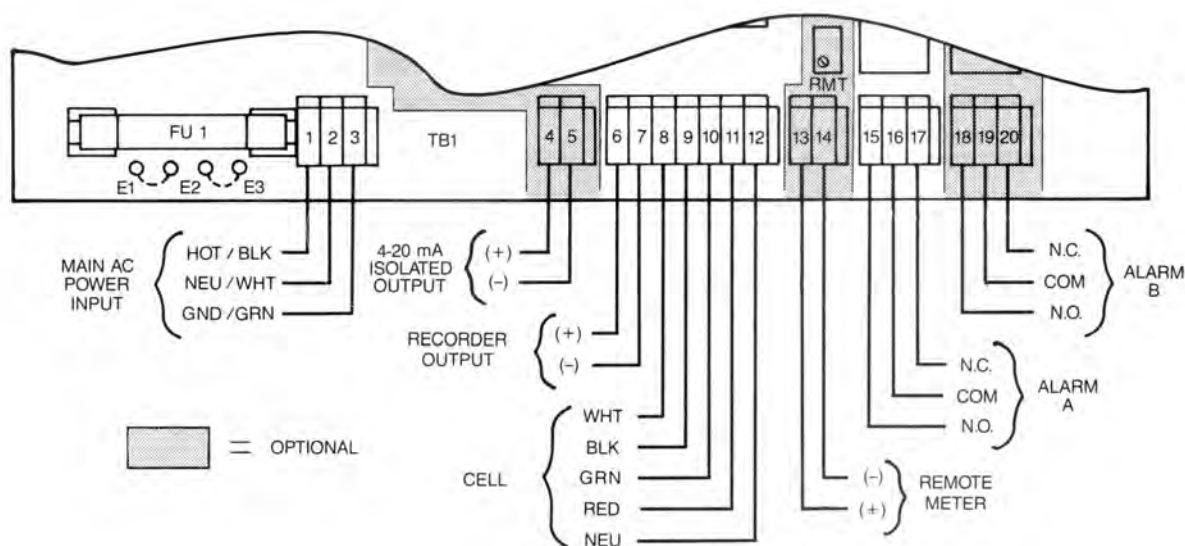
FIG. 2-5 MODEL 767 INSTALLATION DIAGRAM
