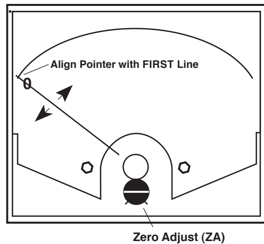
CLEAR PLASTIC COVER (case not shown for clarity) Figure II.G.9
